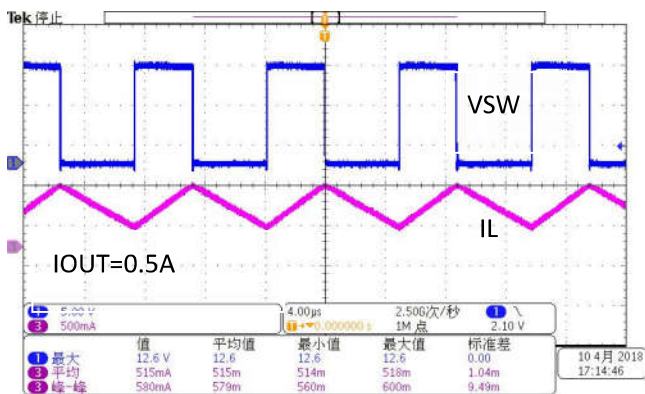
SW VS.Output waveform
