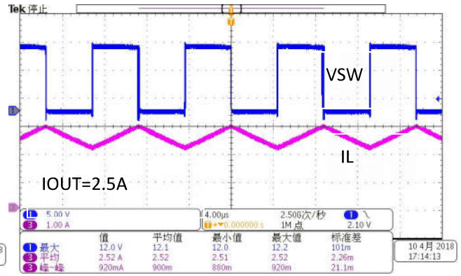
SW VS.Output waveform
