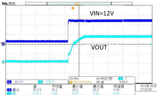
Start-up Waveform
