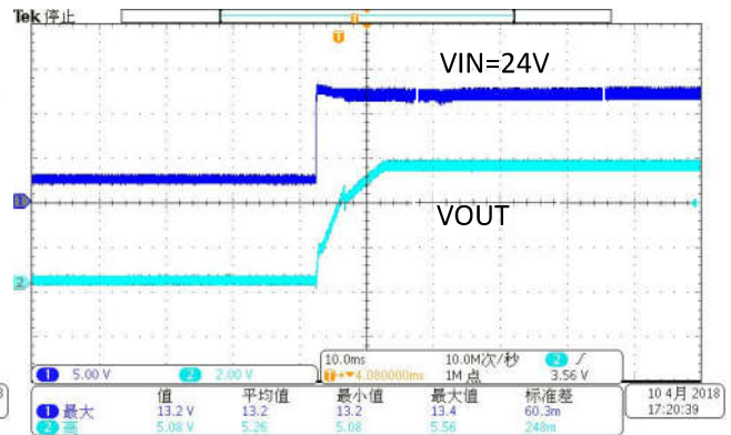
Start-up Waveform
